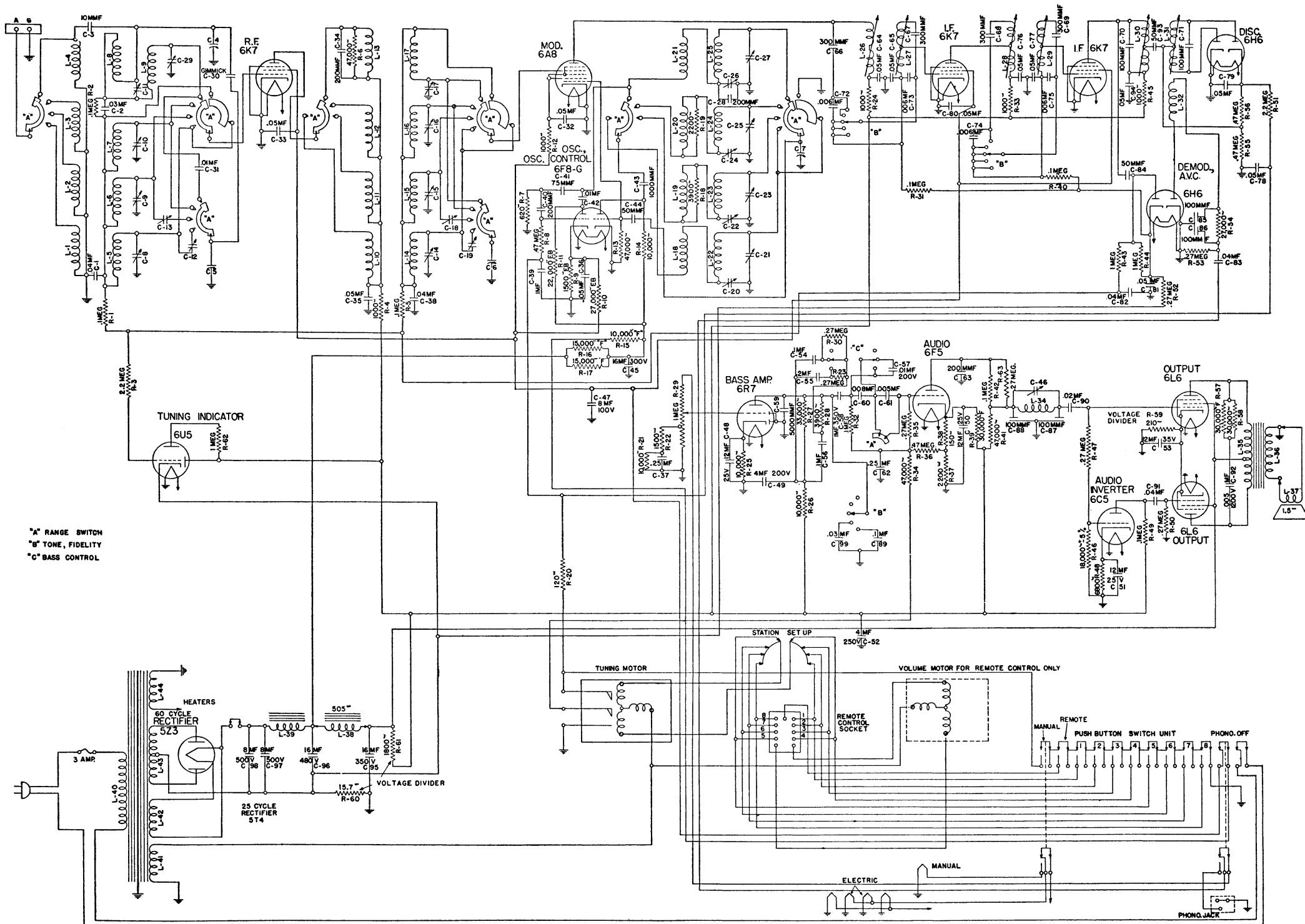
Fig. 2. Schematic Circuit of Receiver.
